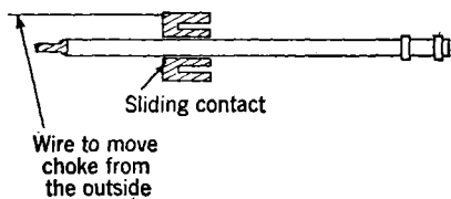
FIG. 18-22.—Movable cathode choke.
